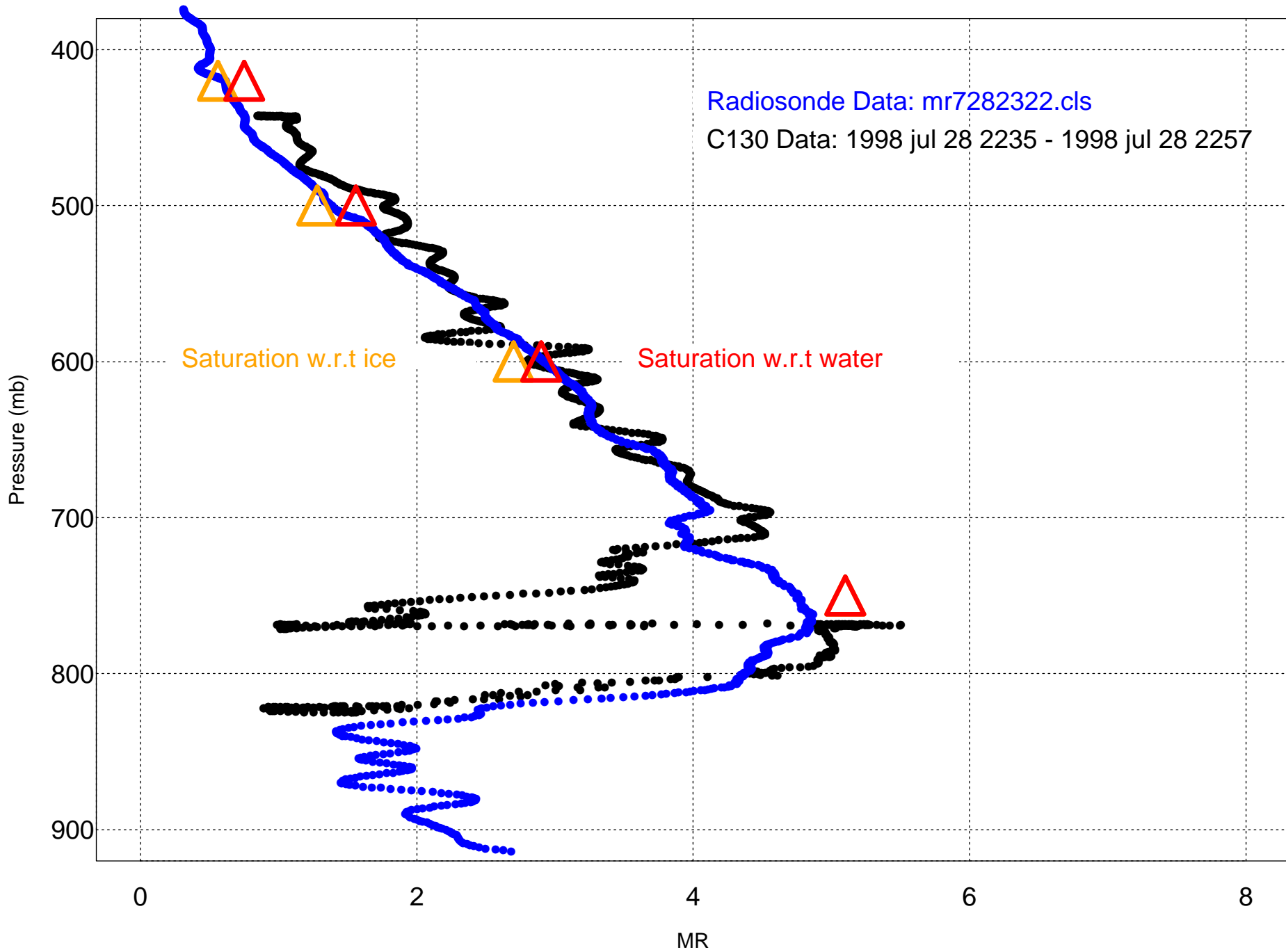
Figure 9: SHEBA 28 July 1998 C130 RF15 Descent - GE Hygrometer vs. Radiosonde
