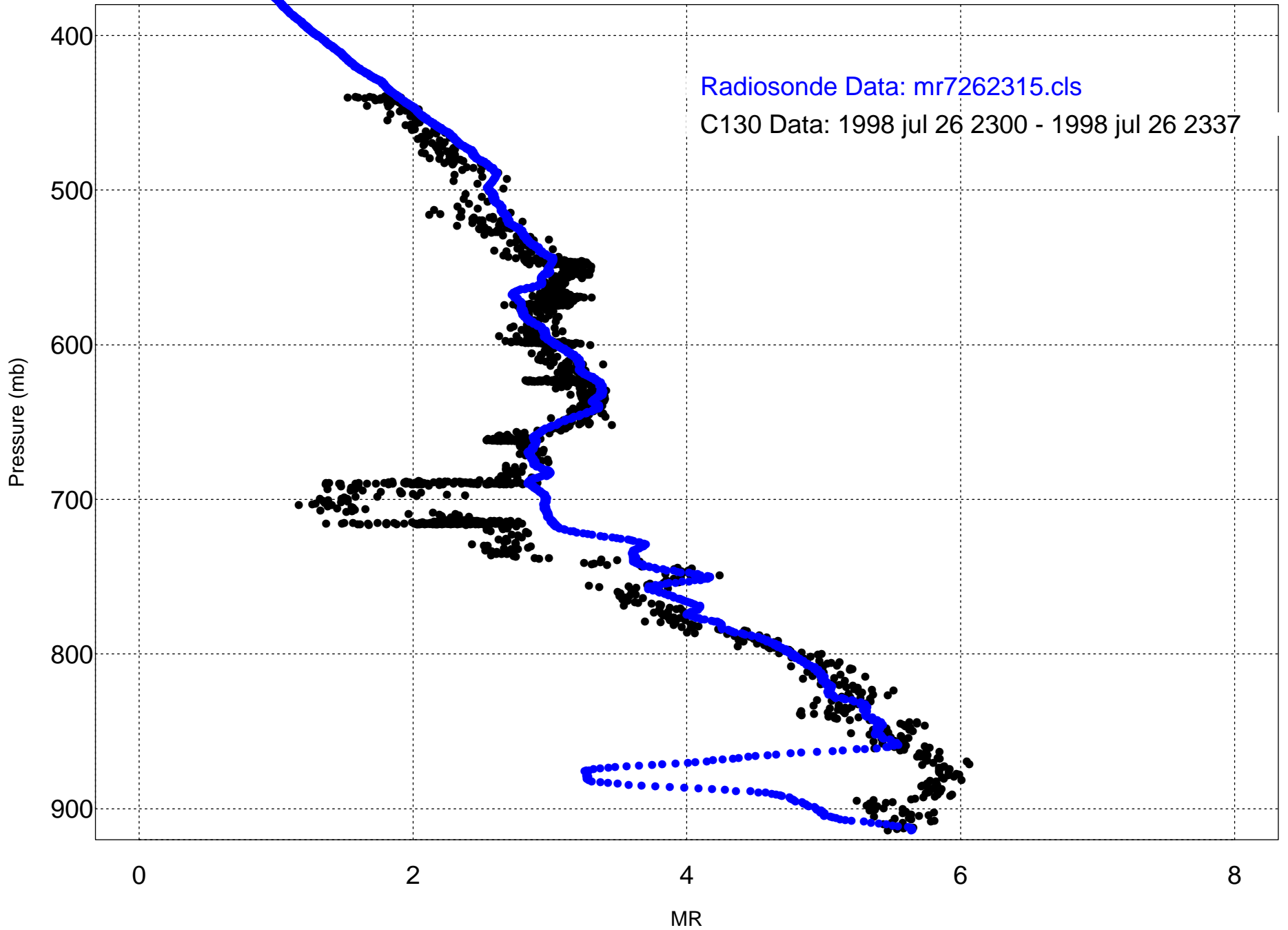
Figure 8: SHEBA 26 July 1998 C130 RF14 Descent - UV Hygrometer vs. Radiosonde
