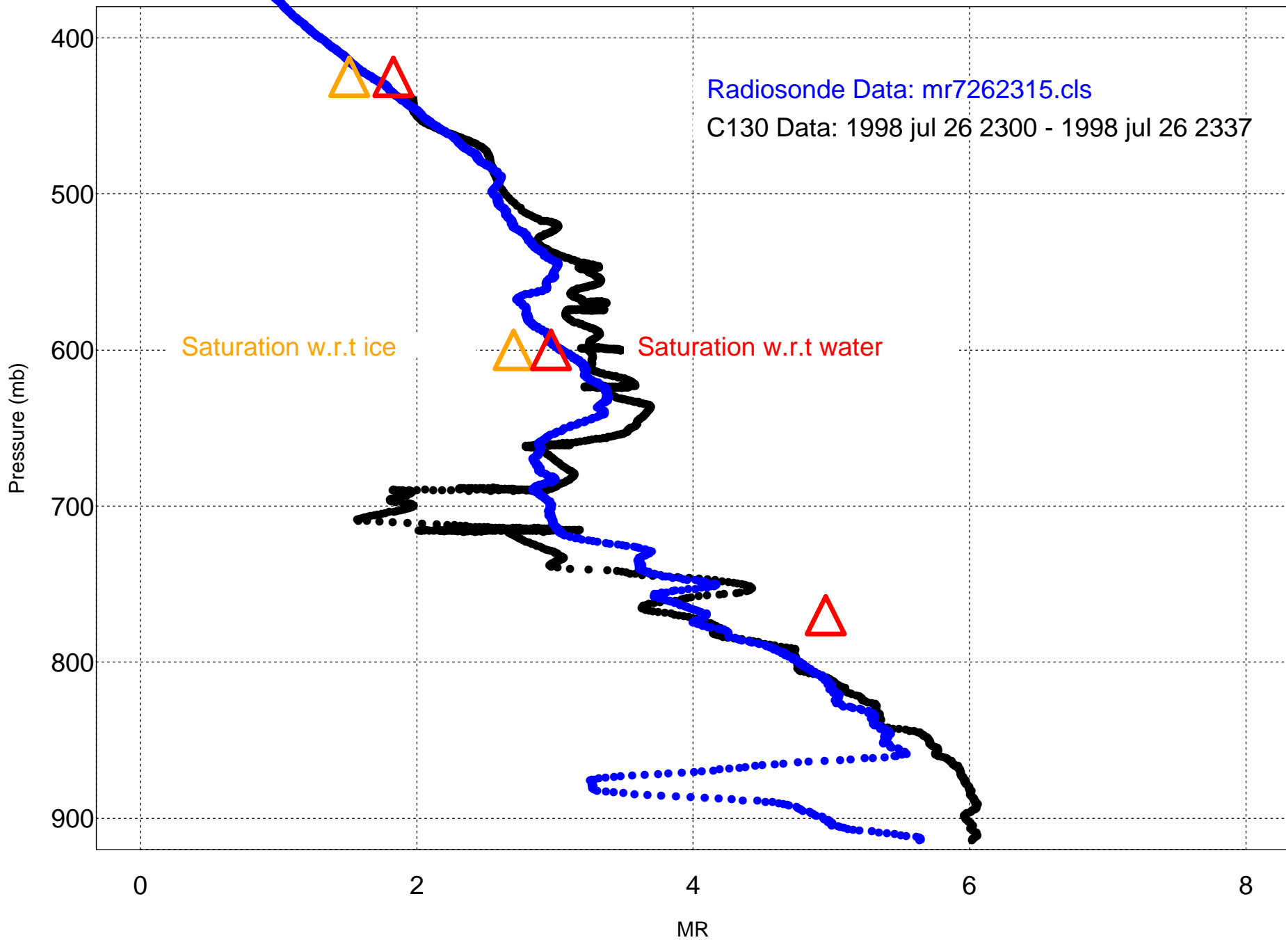
Figure 7: SHEBA 26 July 1998 C130 RF14 Descent - GE Hygrometer vs. Radiosonde
