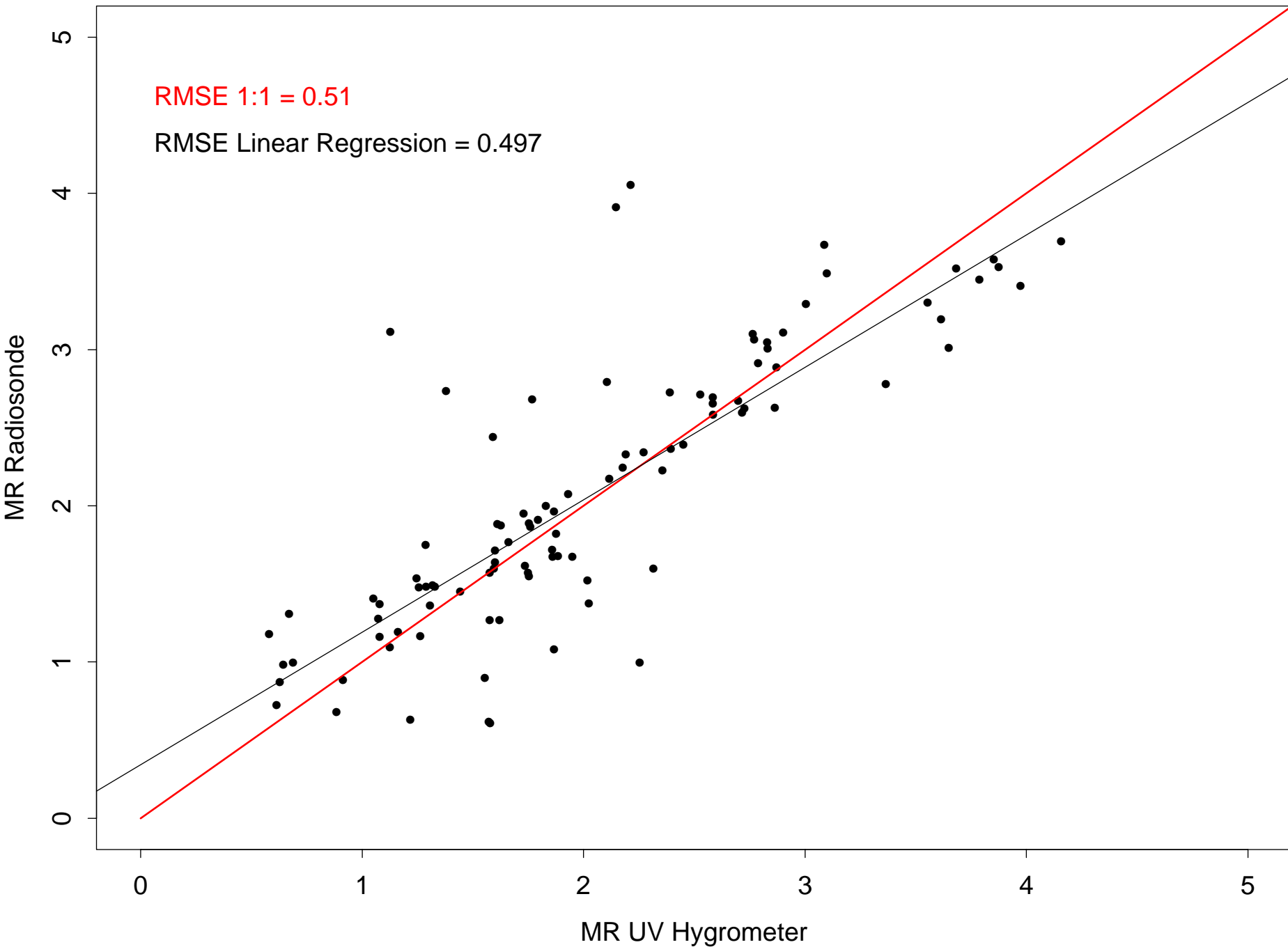
Figure 6B: SHEBA 23 July 1998 C-130 RF13 Mixing Ratio Comparison 500-900 mb
