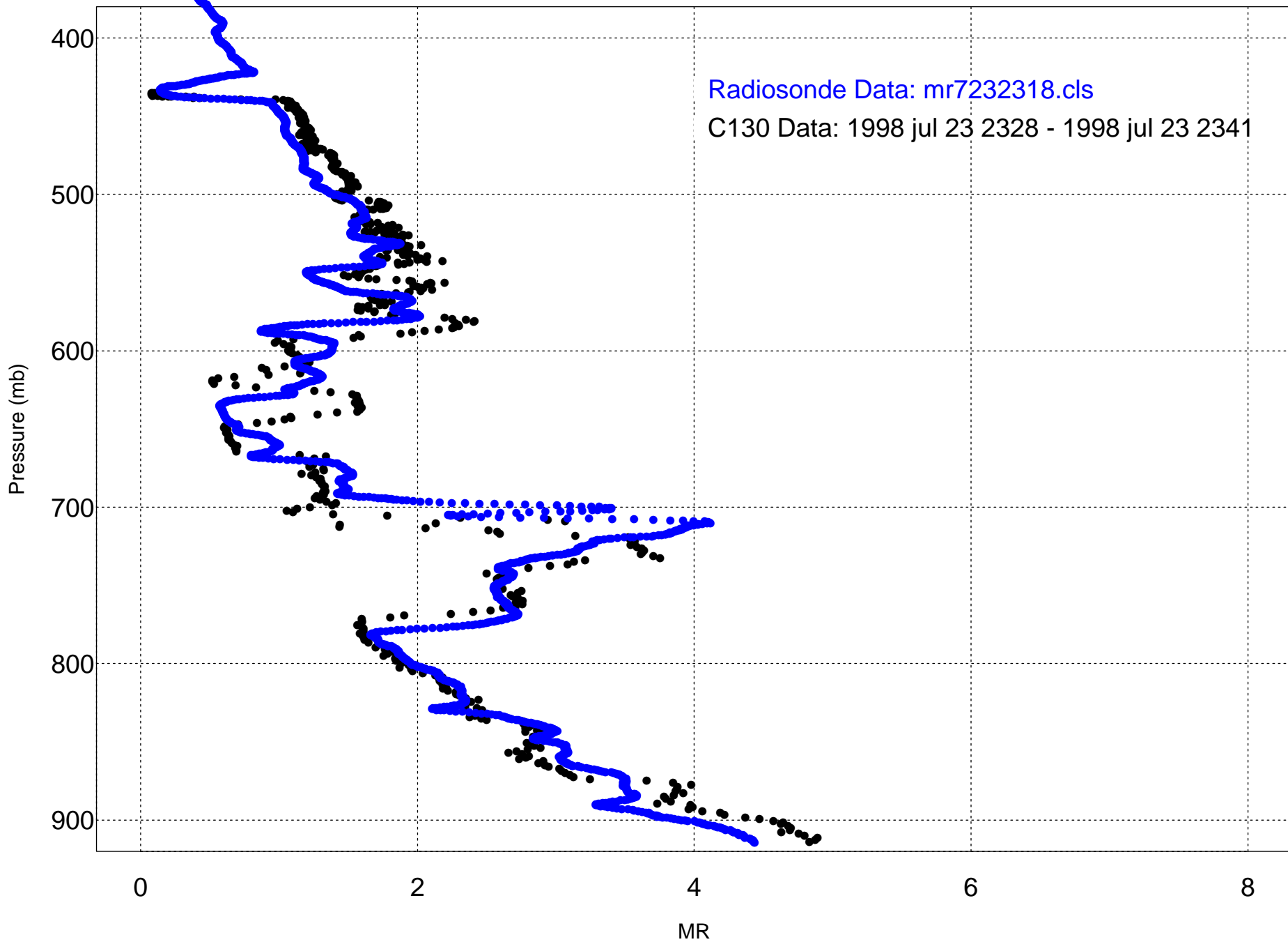
Figure 6: SHEBA 23 July 1998 C130 RF13 Descent - UV Hygrometer vs. Radiosonde
