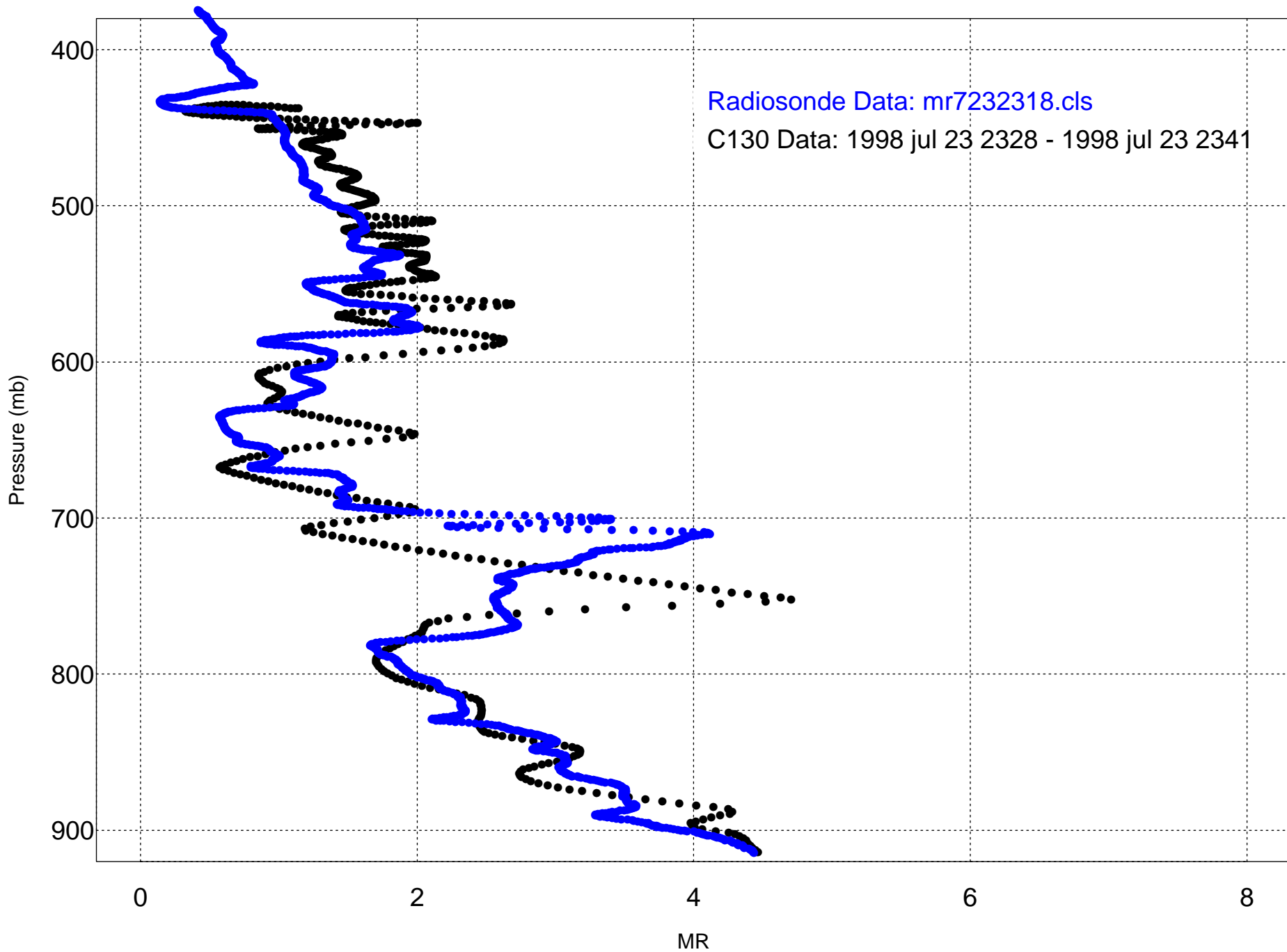
Figure 5: SHEBA 23 July 1998 C130 RF13 Descent - GE Hygrometer vs. Radiosonde
