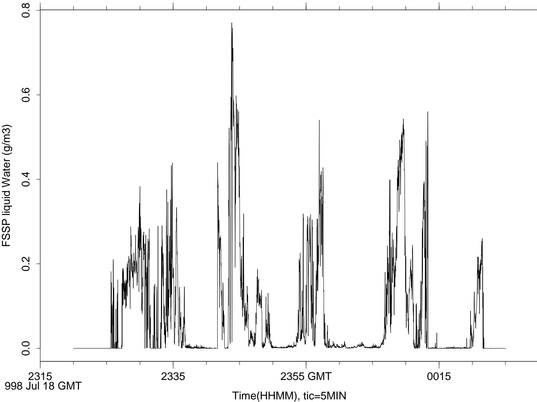
Figure 4: SHEBA 18 July 1998 C130 RF11 Descent and Ascent
