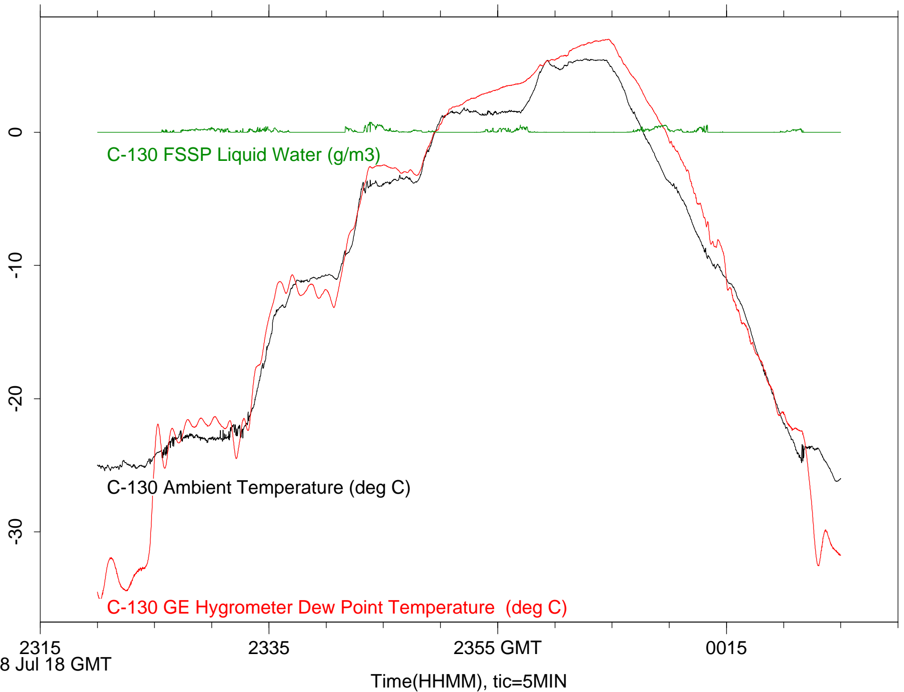
Figure 3: SHEBA 18 July 1998 C-130 RF11 Descent followed by Ascent
