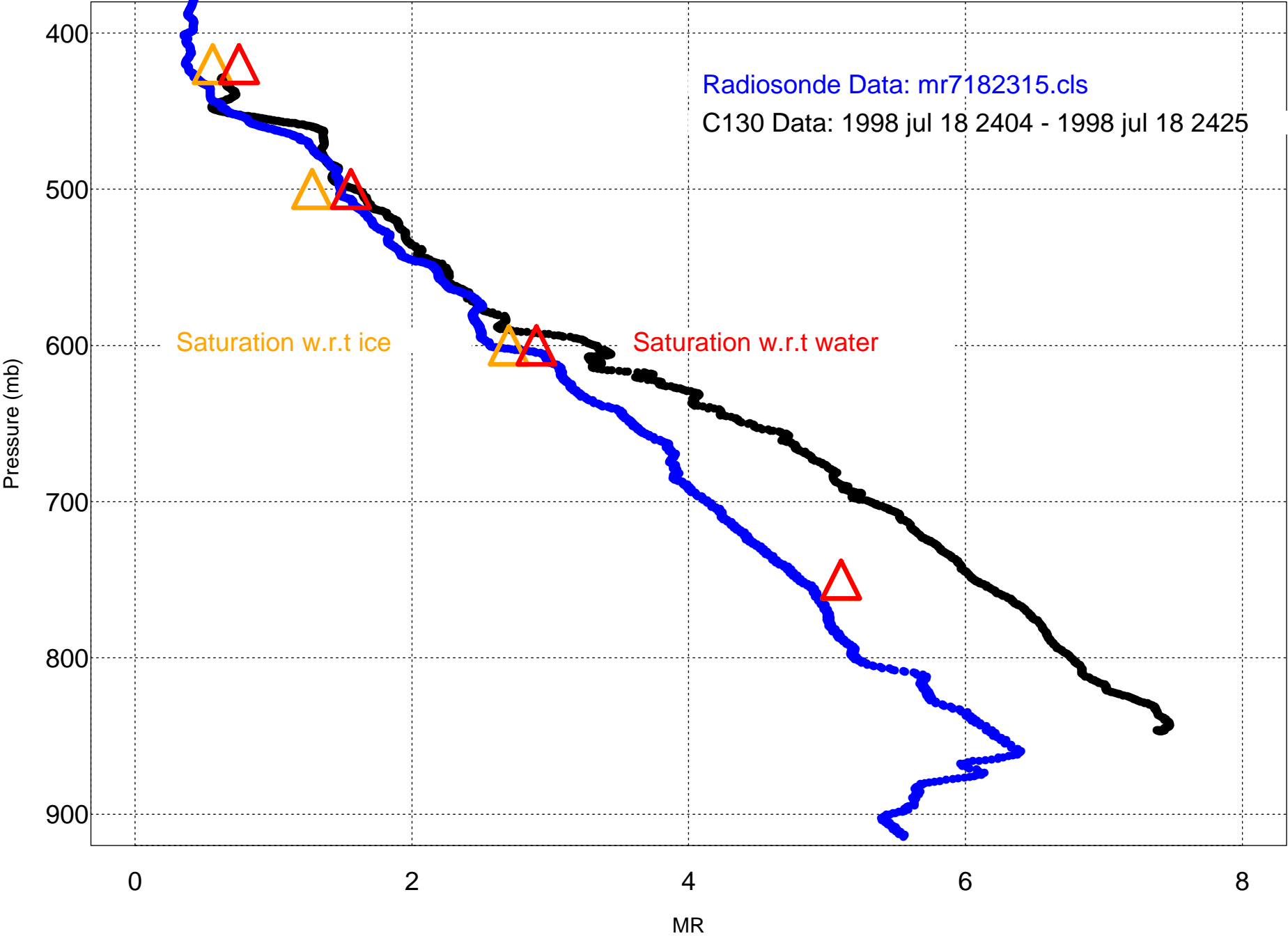
Figure 2: SHEBA 18 July 1998 C130 RF11 Ascent - GE Hygrometer vs. Radiosonde
