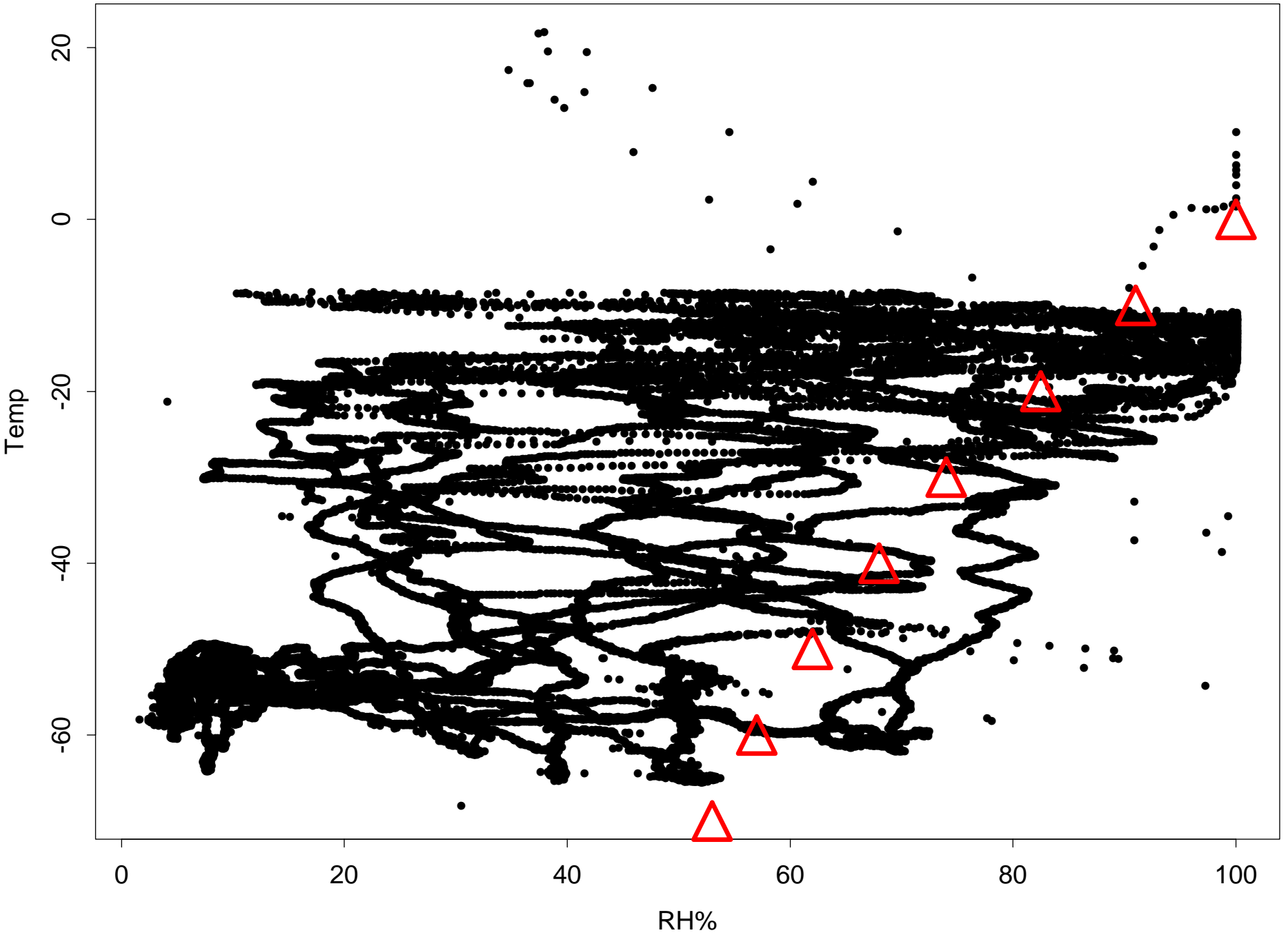
Figure 11: Sheba nov97 : uncorrected soundings
