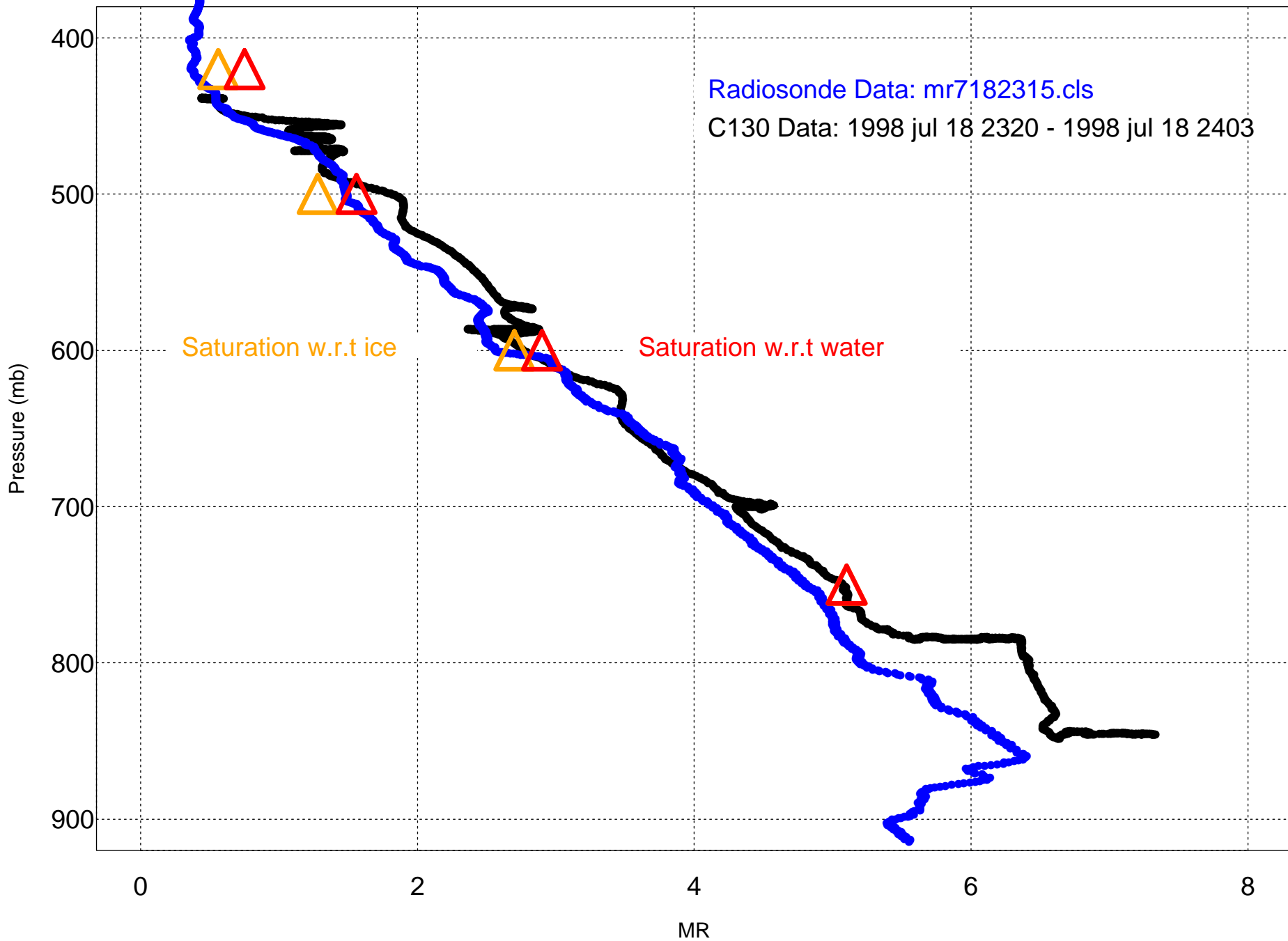
Figure 1: SHEBA 18 July 1998 C130 RF11 Descent - GE Hygrometer vs. Radiosonde
