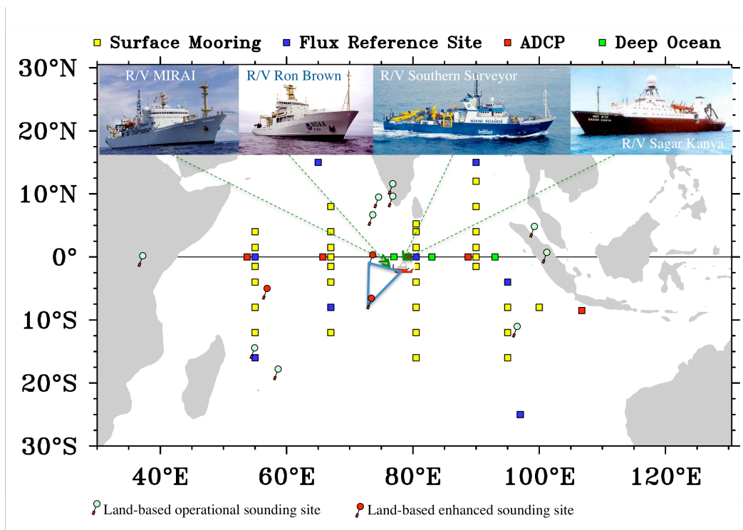
Figure 2 CINDY2011 observing network. The triangle illustrates an option of the sounding-radar array formed by Gan Island, Diego Garcia, and four ships on station in relay. Squares are IndoOS and RAMA moorings.
