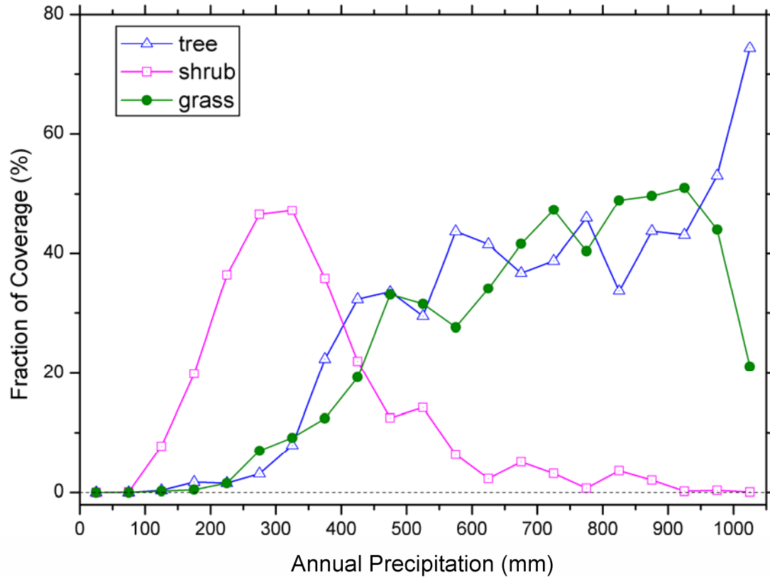
The fraction of vegetation coverage vs. annual precipitation
