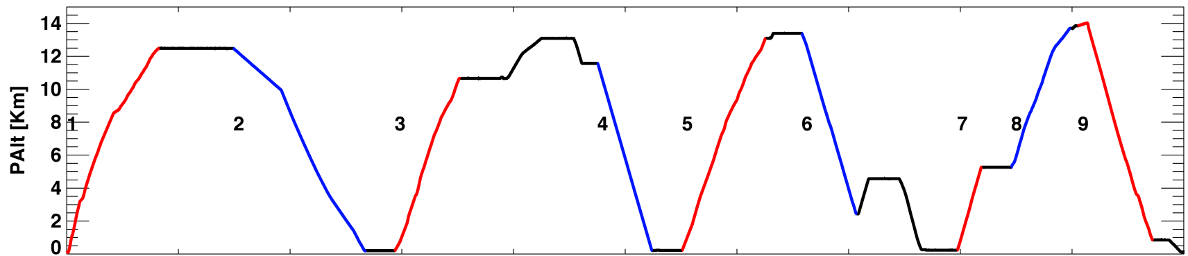
rf07 20140128 Profile Identifications
