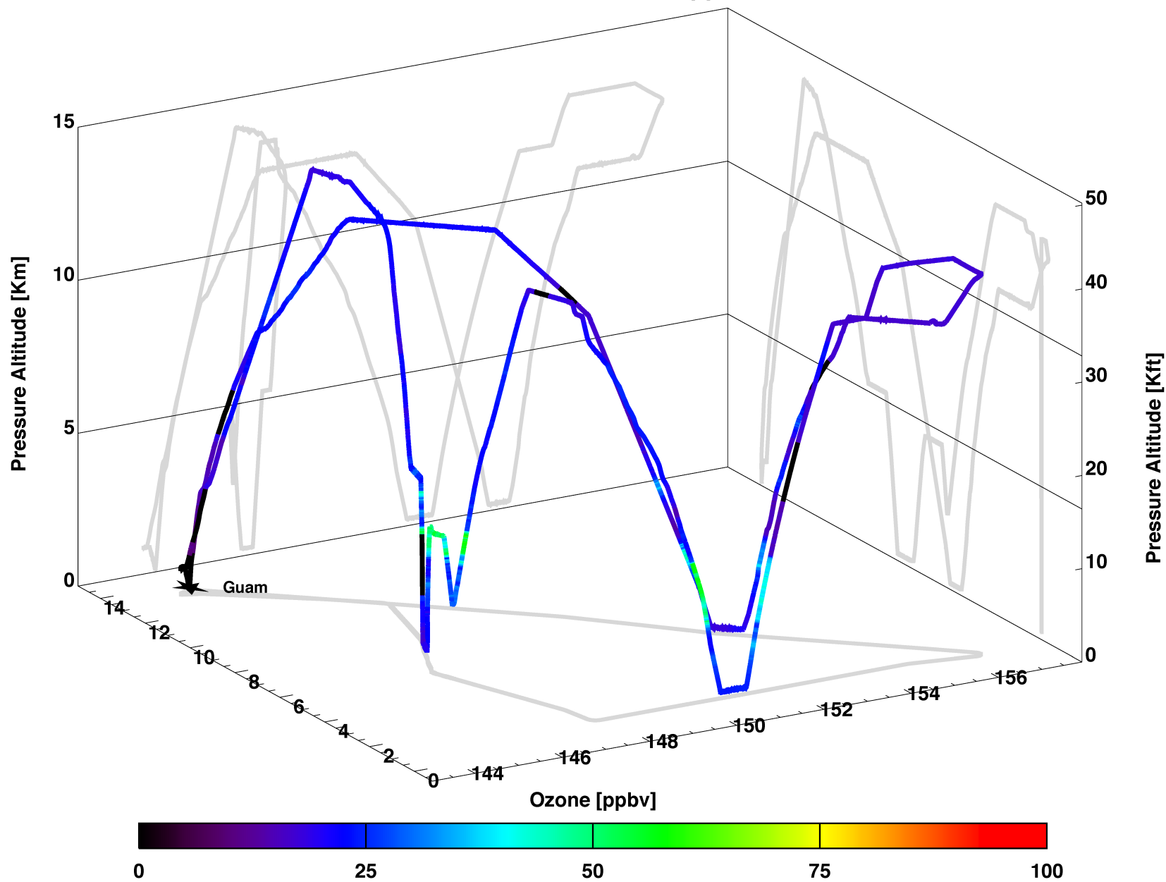
rf07 20140128 Ozone [ppbv]
