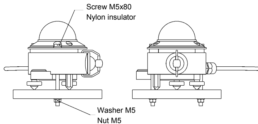
Figure 7 Mounting the pyranometer.
