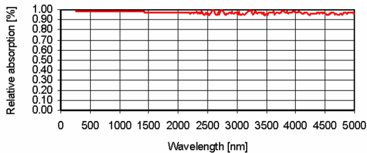
Figure 5 CM 21 Black absorbers relative absorption [%]
