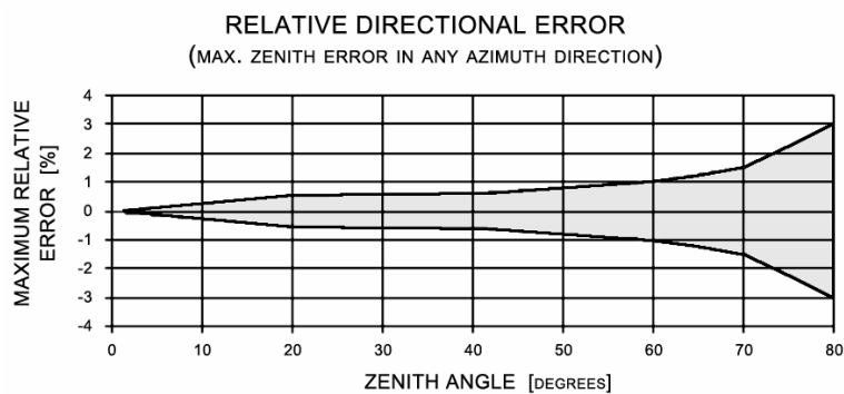
Figure 4 Relative directional error is van CM 21.
