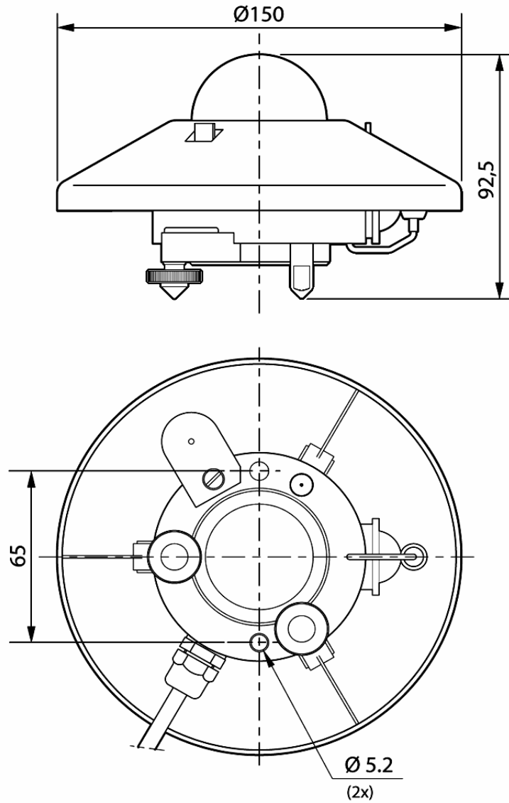
Figure 2 CM 21 Pyranometer outline dimensions in mm.
