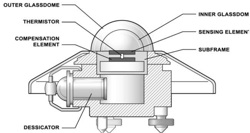
Figure 1 Construction details of a CM 21 pyranometer
