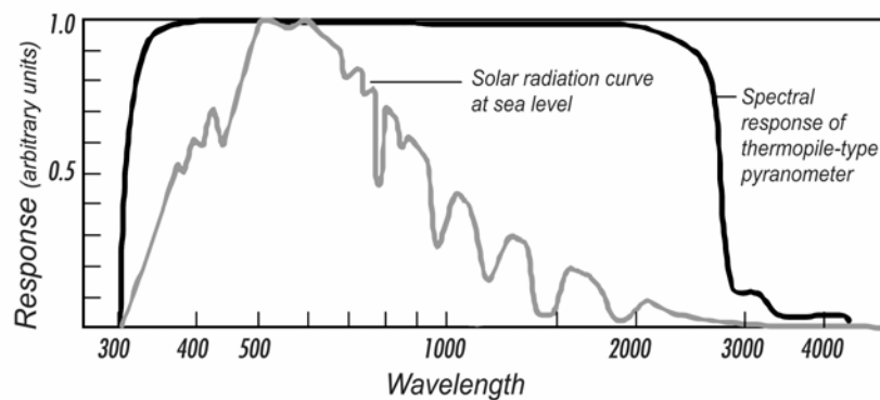
Figure 6 Spectral Response of solar radiation at sea level. Sun at zenith (airmass 1).
