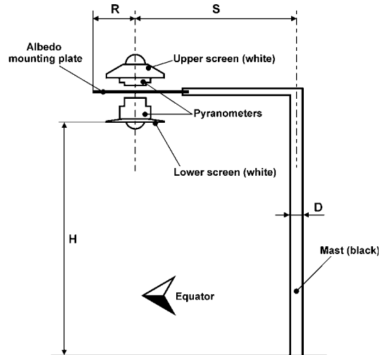
Figure 10 Albedo measurement construction
