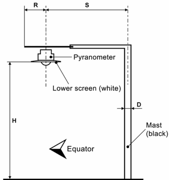
Figure 8 Arrangement to measure reflected global radiation
